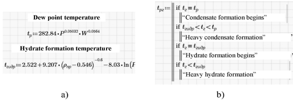
Fig. 1. Screenshots of modelling in MathcadPrime software
