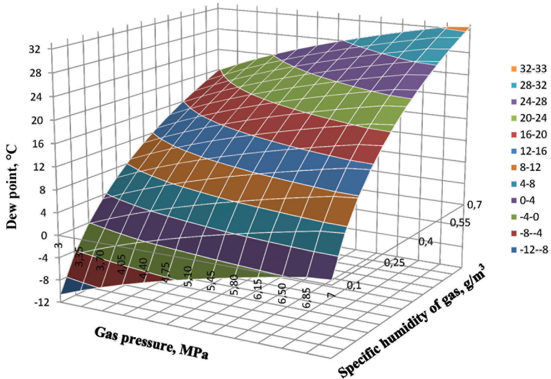
Fig. 2. Dependence of the dew point (°C) on gas pressure and specific humidity
