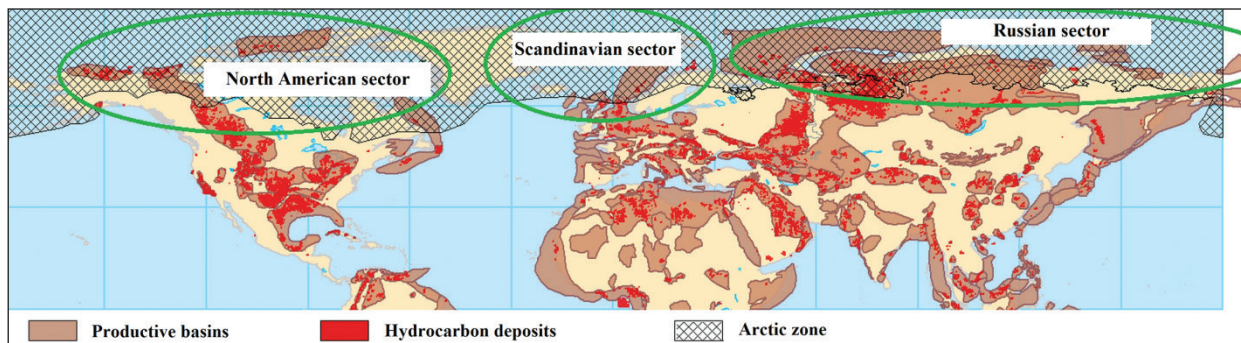
Fig. 1. Oil-and-gas bearing zoning of the Arctic region
