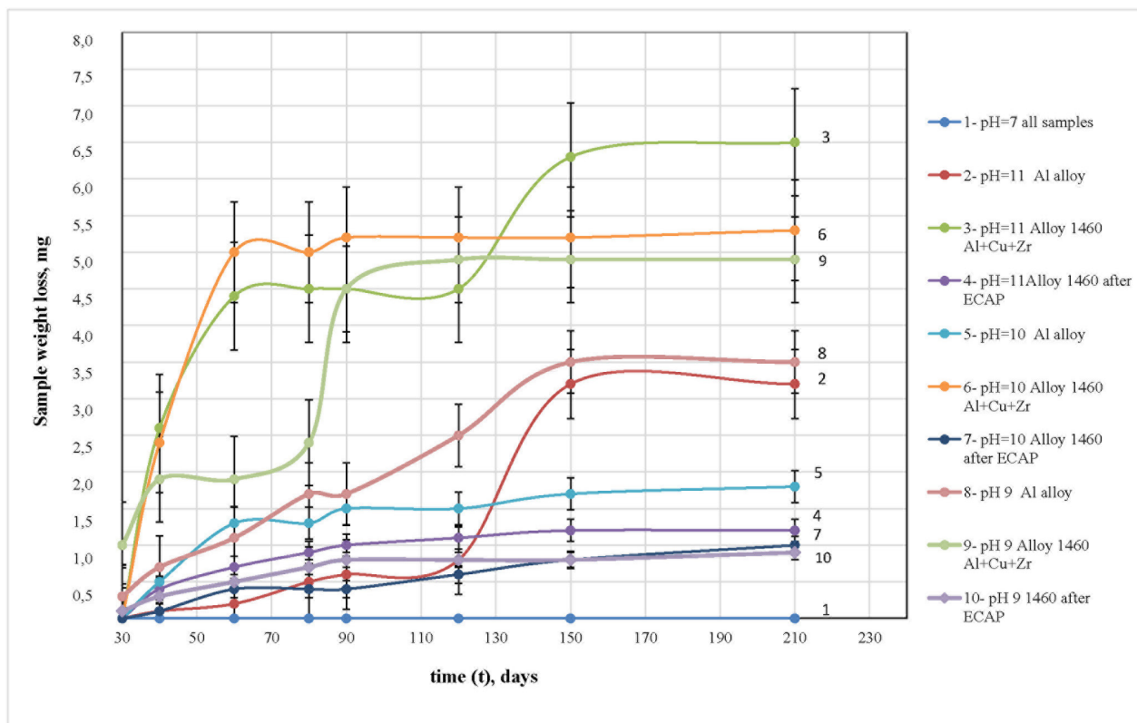
Fig. 4. Weight loss vs. time of exposure to aggressive media curves
