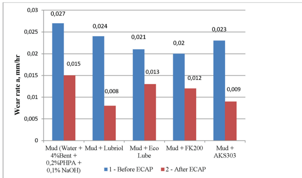
Fig. 3. Wear rate for alloy 1420 samples with coarse grain and SMC structure at T=293 K in drill fluid with different lubricating additives (confidence intervals established at 80% probability). (These results were obtained on friction machine UMT-2168)
