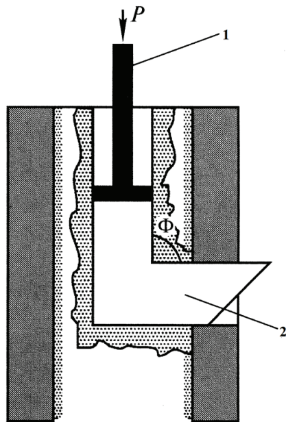
Fig. 1. Diagram of equal channel angular pressing: 1) piston, 2) pipe strip
