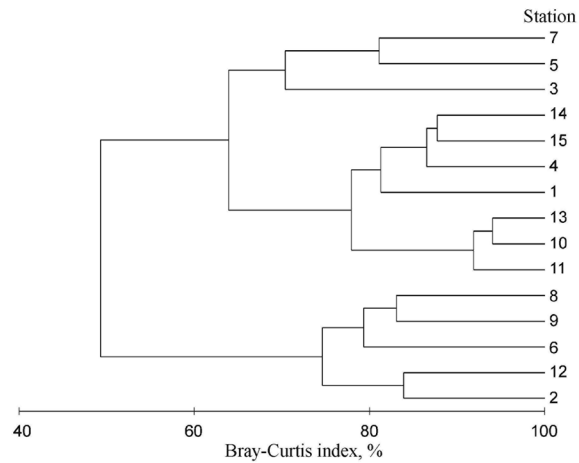
Fig. 2. Dendrogram of station similarity in terms of zooplankton count in the central part of the Barents Sea in November 2010
